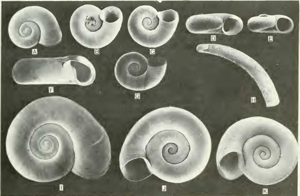
FIG. 15. SEM photos of Coahuilix hubbsi , Coahuilix landyei and Orygoceras (?) sp. Shells A–E are Coahuilix hubbsi from Locality 64; shells F, G, I, J, K are paratypes of Coahuilix landyei (ANSP 355211) from Locality 64; and shell H is Orygoceras (?) sp. from Locality 67. Shell A is 0.871 mm wide, and all others are printed to the same enlargement except H, the tube of which is 2.26 mm long.
